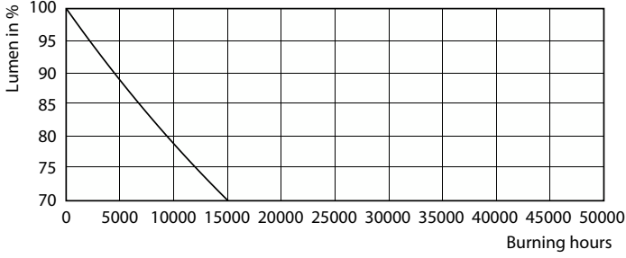
Lumen Maintenance Diagram - ESS LEDspots 50W GU10 840 36D ND TR
